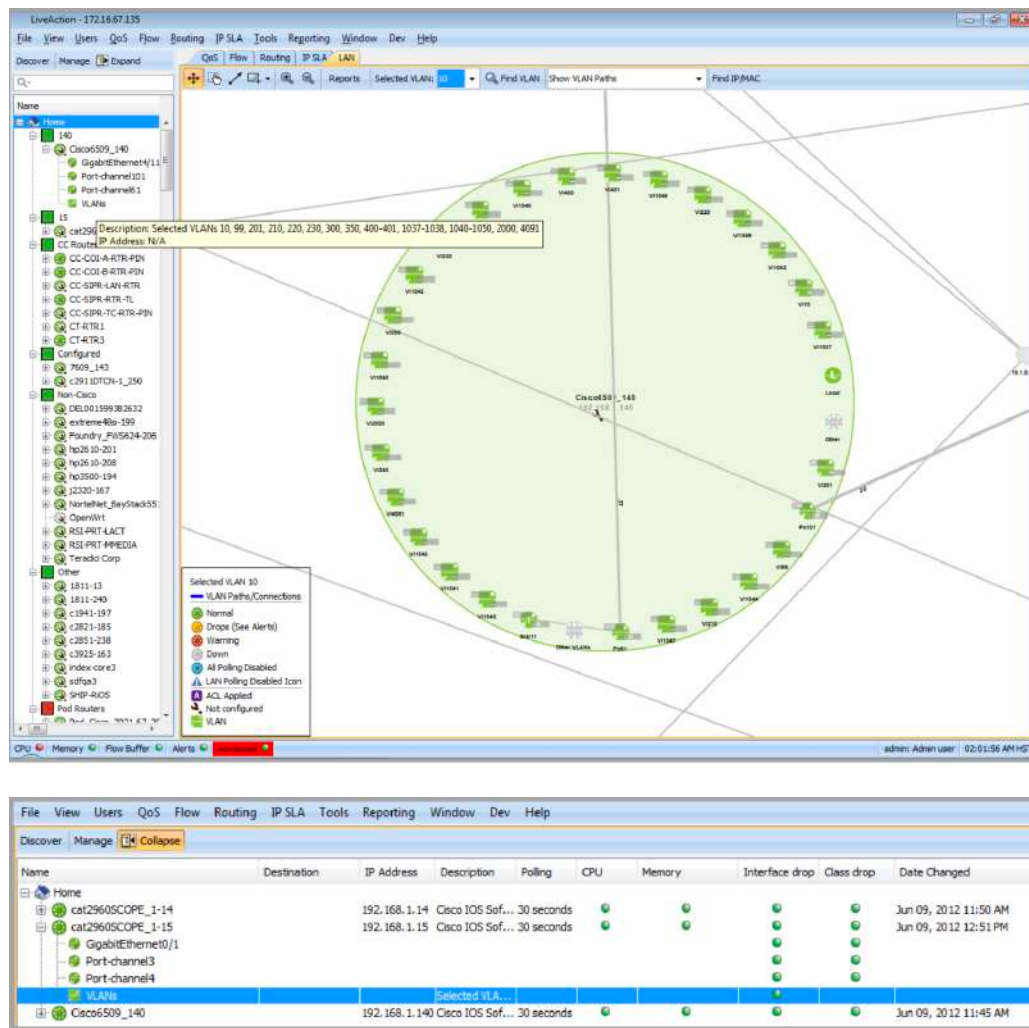
Fig. 10-2: Expanded System Hierarchy View with VLANs
